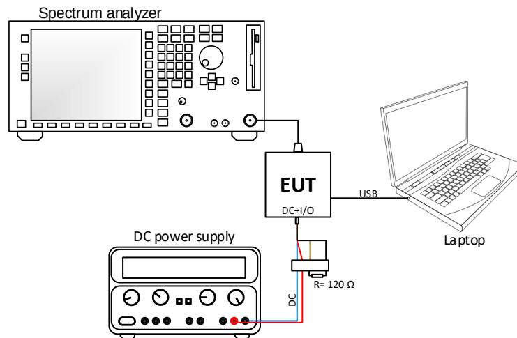
Figure 5.5-2: Antenna port testing block diagram
