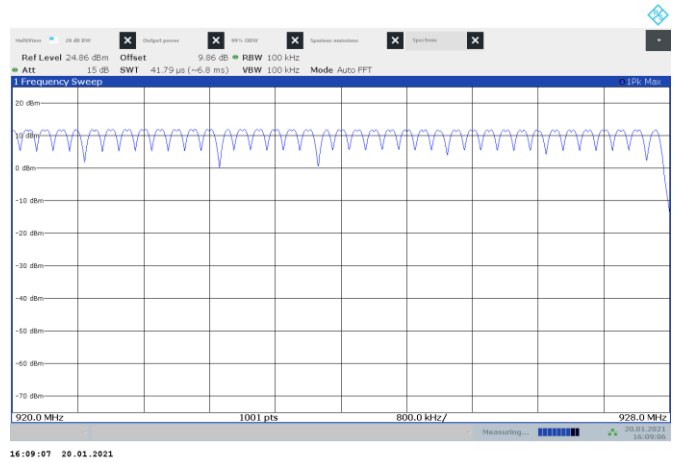
Figure 8.5-8: Number of channels within 920–928 MHz (39.5 of 129), sample plot
