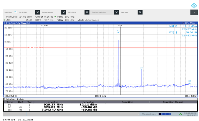
Figure 8.7-12: Conducted spurious emissions on high channel at 150 kbps
