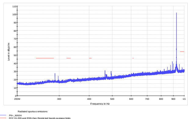
Figure 8.7-18: Radiated spurious emissions within 200–1000 MHz on high channel
