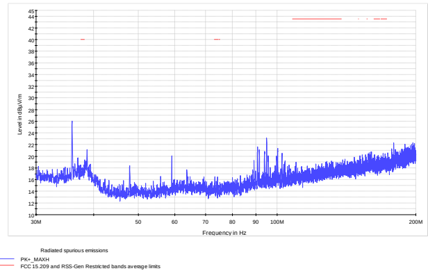
Figure 8.7-14: Radiated spurious emissions within 30–200 MHz on mid channel
