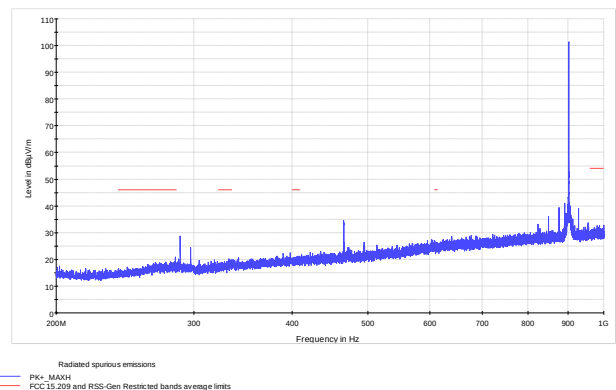
Figure 8.7-16: Radiated spurious emissions within 200–1000 MHz on low channel
