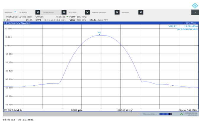
Figure 8.6-6: Output power on high channel, 150 kbps
