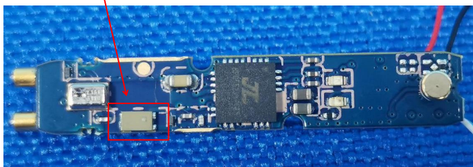
Ceramic Antenna
