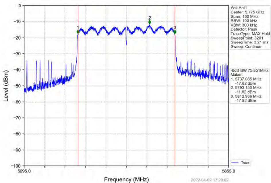
802.11ac(VHT80)_MCH_5775MHz_Ant1_NTNV
