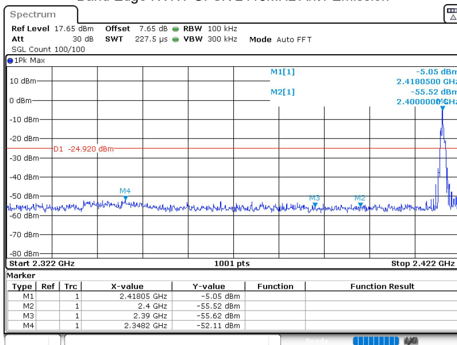
Band Edge NVNT GFSK 2418MHz Ant1 Emission
