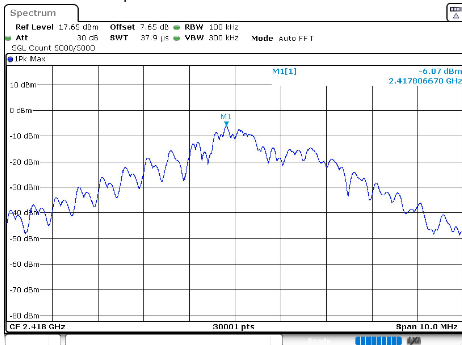
Tx. Spurious NVNT GFSK 2418MHz Ant1 Ref
