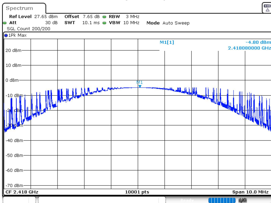
Power NVNT GFSK 2418MHz Ant1
