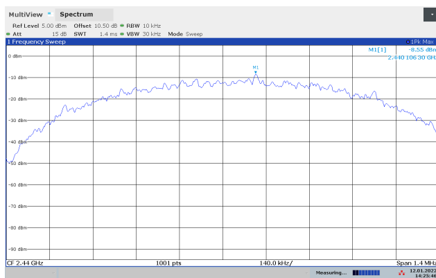
PSD, 2440 MHz
