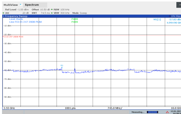
Conducted Emissions 2.55-10 GHz, 2402 MHz
