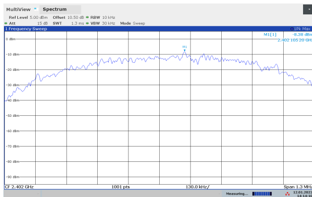
PSD, 2402 MHz
