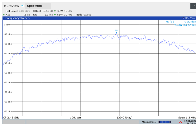
PSD, 2480 MHz
