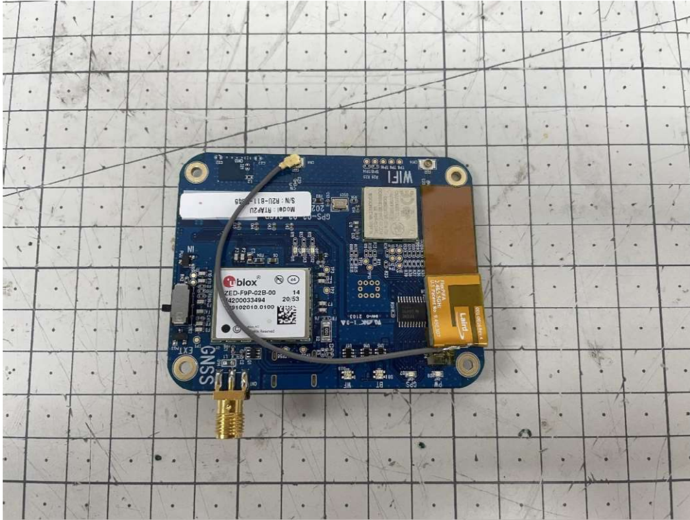
Top board Front
