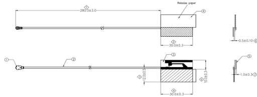
Antenna Drawing
