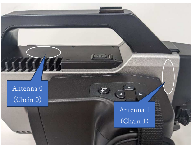
Antenna Positions
