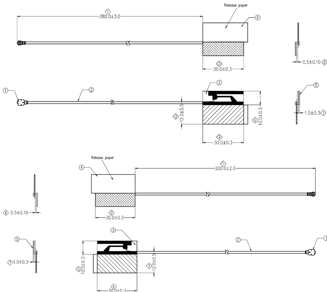
Antenna Drawing (Different cable length)
