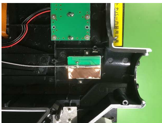
Antenna in Enclosure
