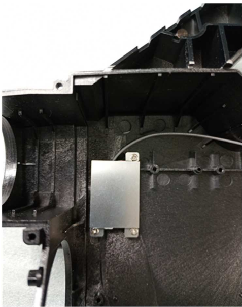
Antenna 1 in Enclosure
