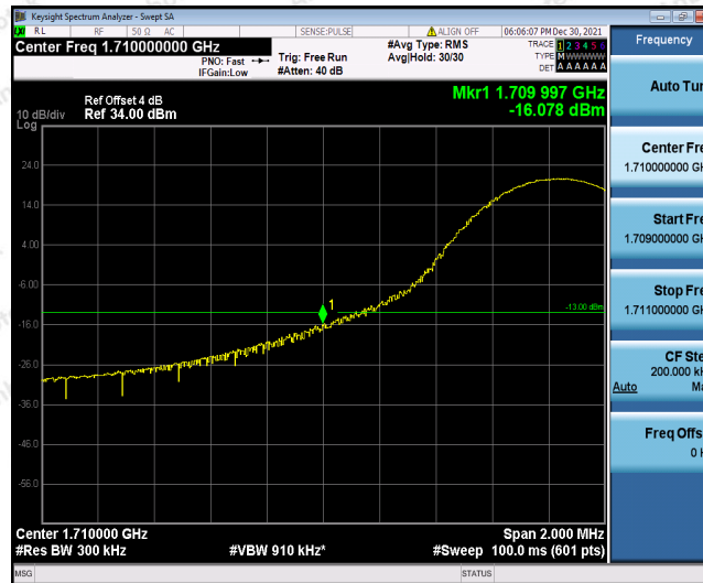
Band66-15MHz-QPSK-132047-1RB#74
