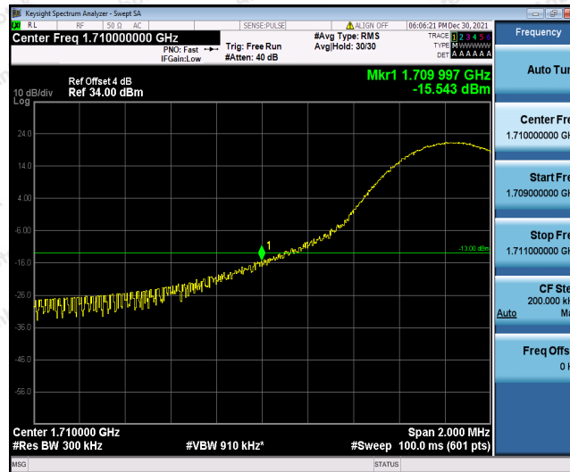
Band66-15MHz-16QAM-132047-1RB#74
