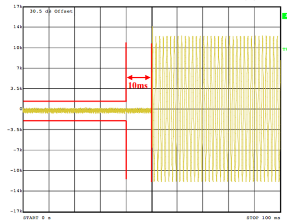
Transmitter Frequency Behavior @ 12.5 KHz Channel Separation-----On – Off
