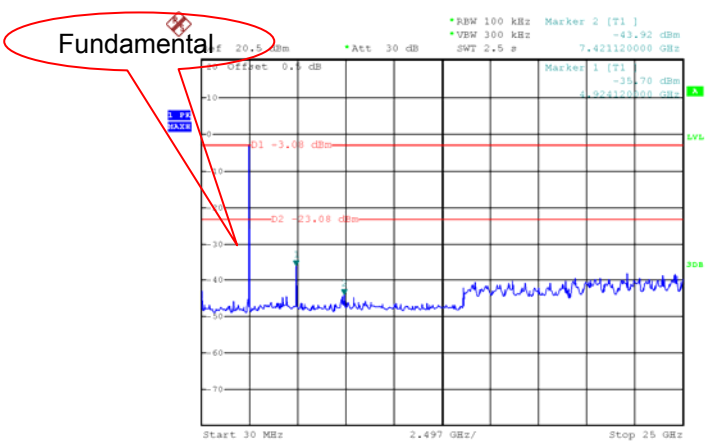
Mode: channel 39
