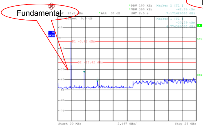
Mode: channel 0
