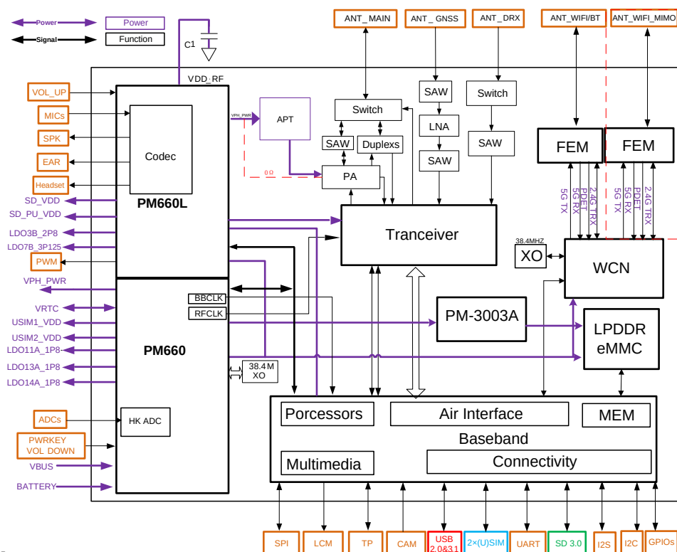
Figure 1: Functional Diagram
