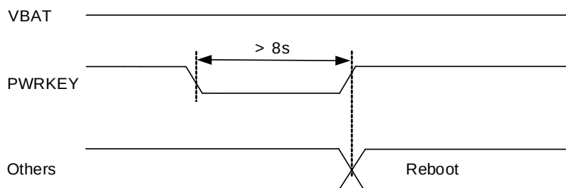
Figure 10: Timing of Rebooting Module
