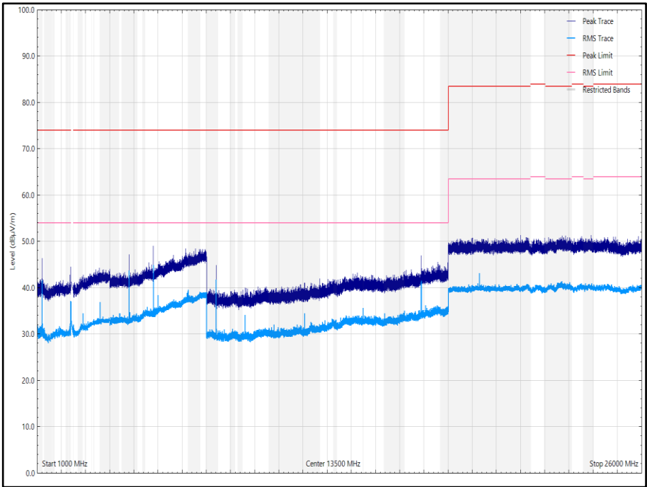
Figure 21 - CH1_802.11b_1Mbps_Y, 2412 MHz, 1 GHz to 26 GHz, Vertical
