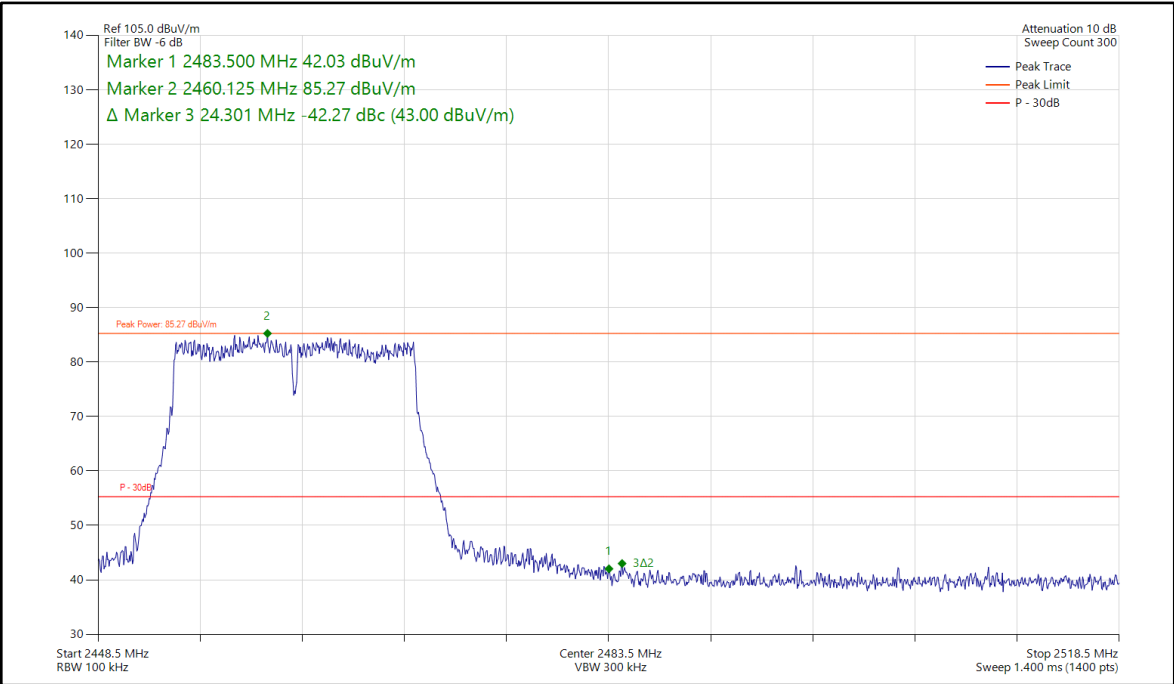
Figure 10 - CH11_802.11g, 2462 MHz, Band Edge Frequency 2483.5 MHz
