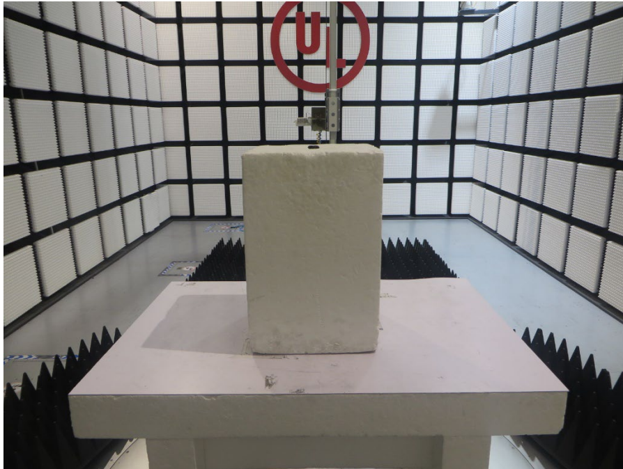
RADIATED EMISSIONS MEASUREMENT SETUP (Above 1G– Y axis)
