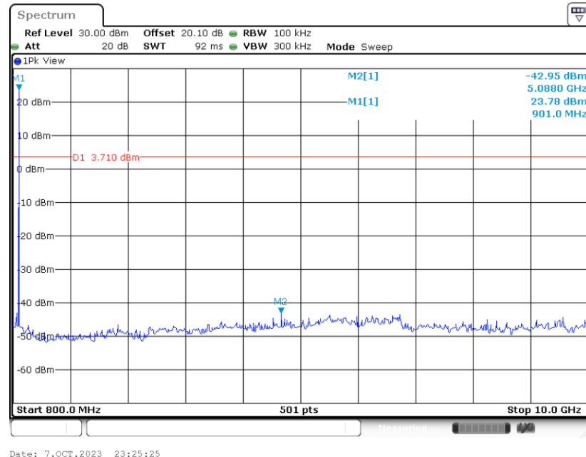
Conducted Spurious Emission Plot on 902.5 MHz
