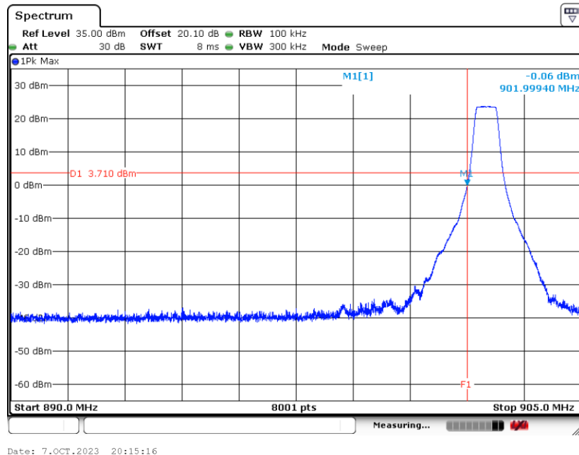
Low Band Edge Plot on 902.5 MHz
