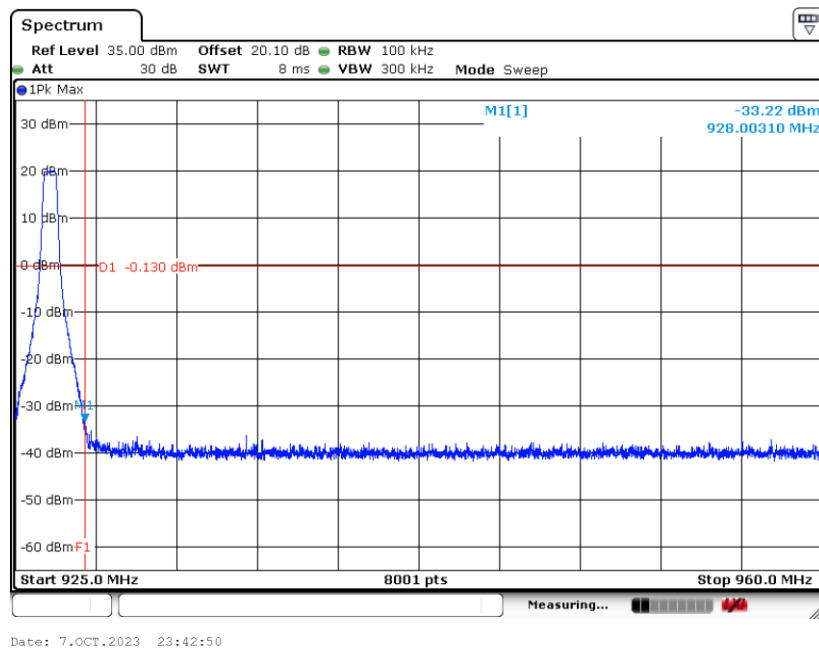
High Band Edge Plot on 926.5 MHz
