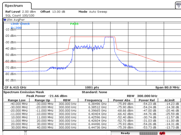
Plot on Channel 6415MHz 52RU40
