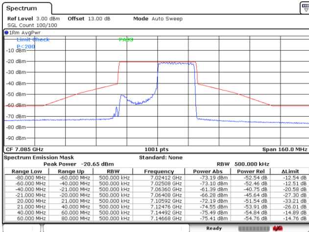
Plot on Channel 7085MHz 242RU62
