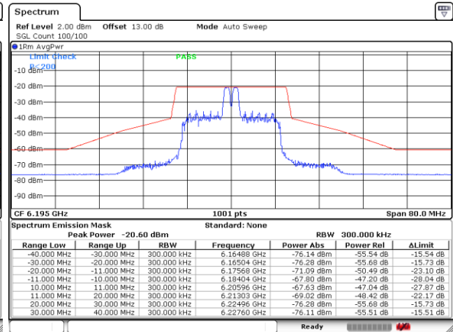
Plot on Channel 6195MHz 26RU4
