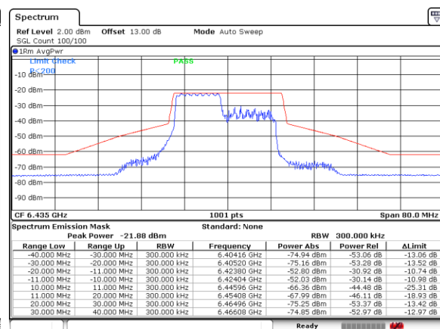
Plot on Channel 6435MHz 106RU53
