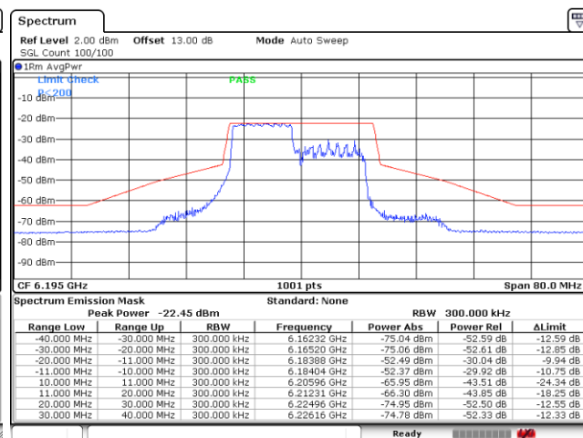
Plot on Channel 6195MHz 106RU53
