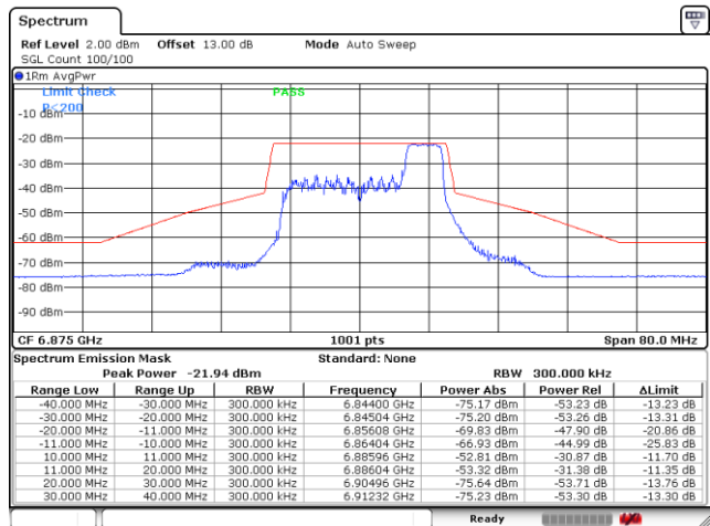
Plot on Channel 6875MHz 52RU40
