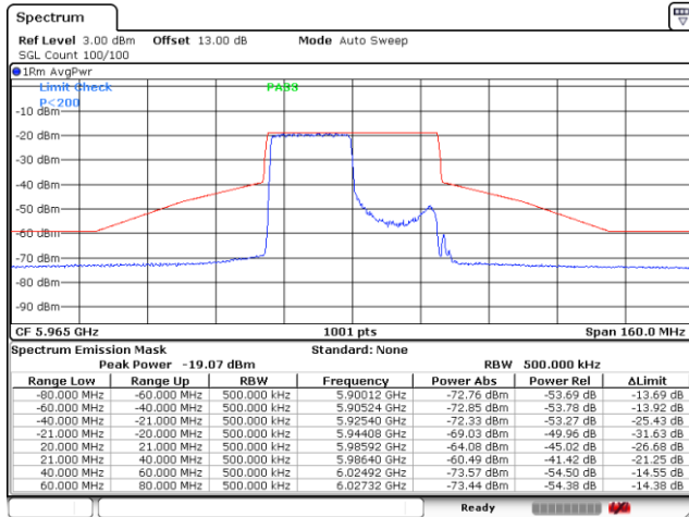
Plot on Channel 5965MHz 242RU61
