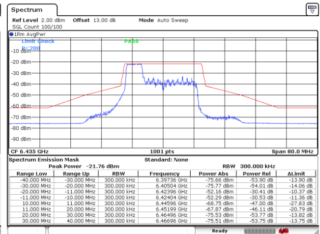
Plot on Channel 6435MHz 52RU37
