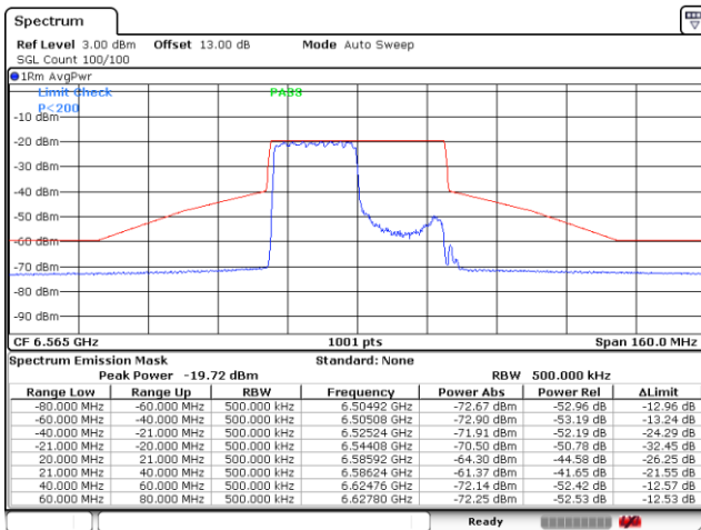
Plot on Channel 6565MHz 242RU61
