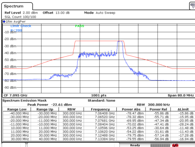
Plot on Channel 7095MHz 26RU8
