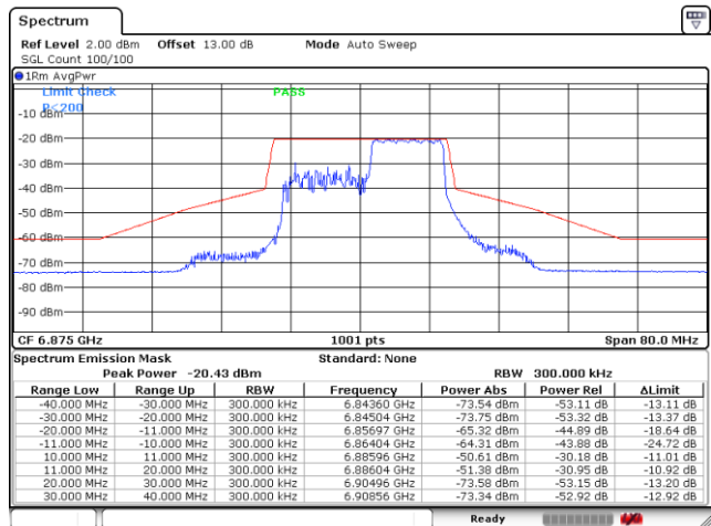
Plot on Channel 6875MHz 106RU54
