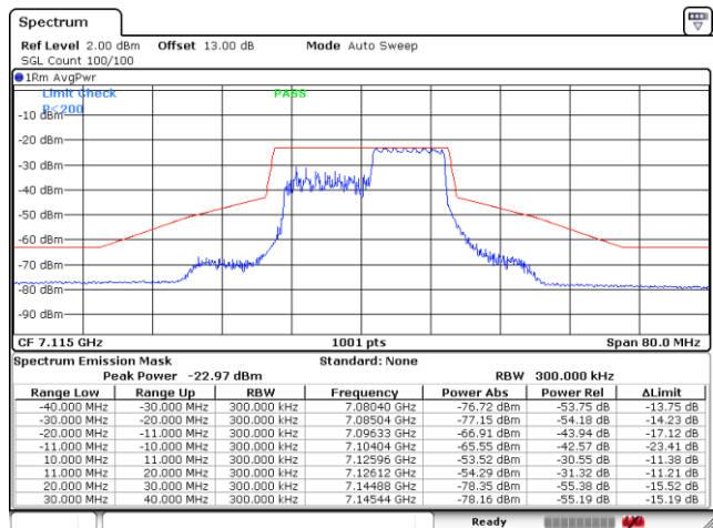
Plot on Channel 7115MHz 106RU54
