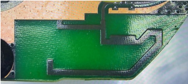
Wi-Fi antenna
