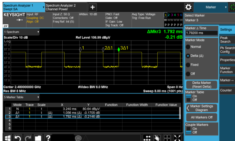
Zigbee mode for Sample 2
