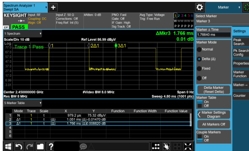
Zigbee mode for Sample 1
