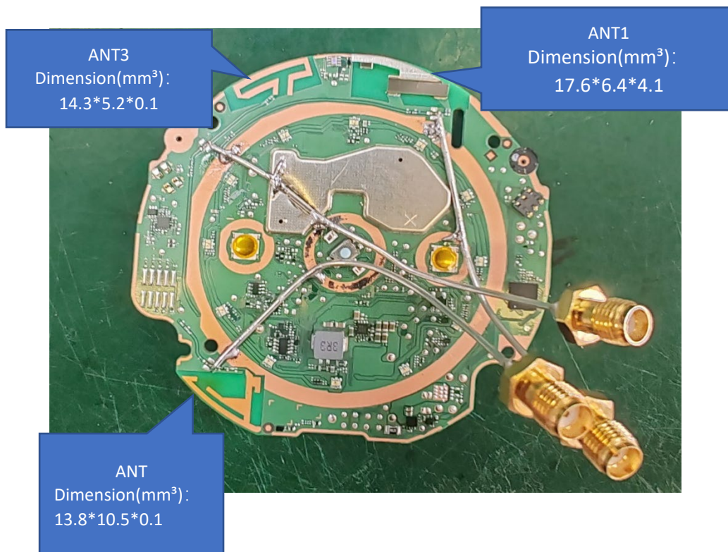
Antenna Photo with Antenna Dimensions
