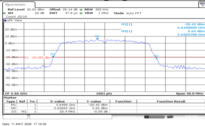
11N20SISO_Ant1_5660
