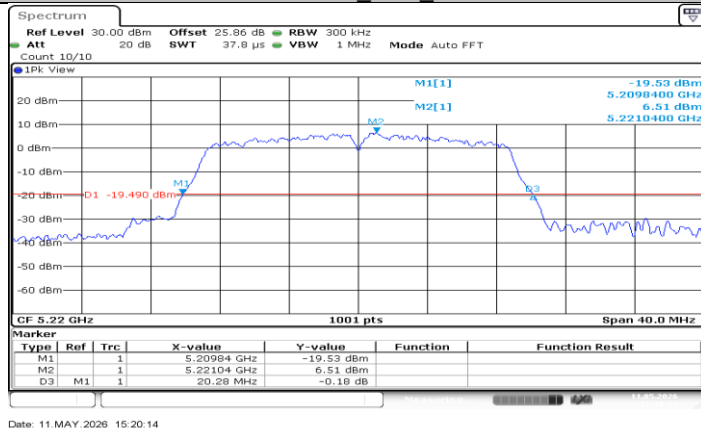
11N20SISO_Ant1_5220
