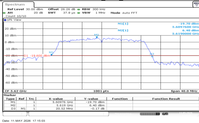
11N20SISO_Ant1_5620
