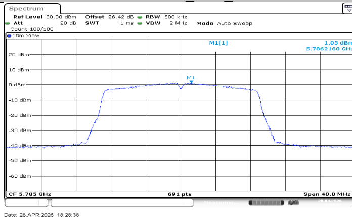
11AC20SISO_Ant1_5785
