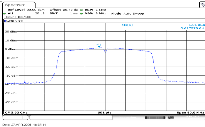
11N40SISO Ant1_5630
