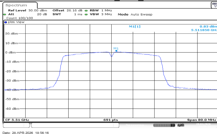
11AC40SISO_Ant1_5510
