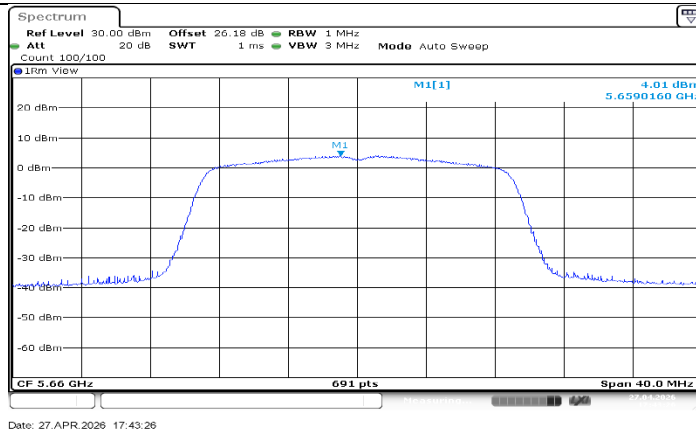
11N20SISO Ant1_5660
