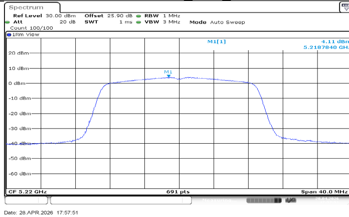
11AC20SISO_Ant1_5220
