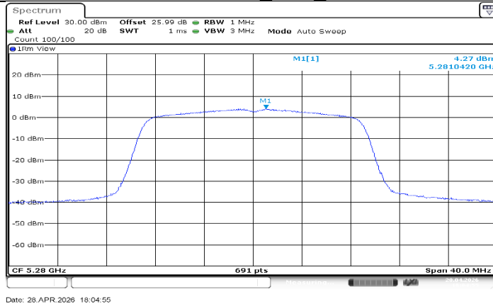
11AC20SISO_Ant1_5280
