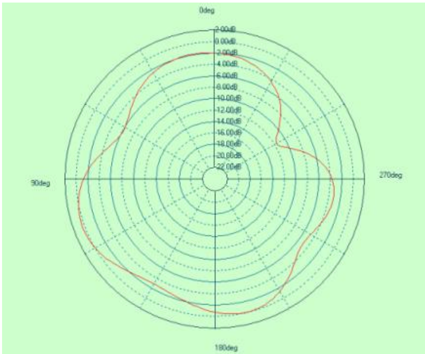
2. 2440MHz 2D-E1
