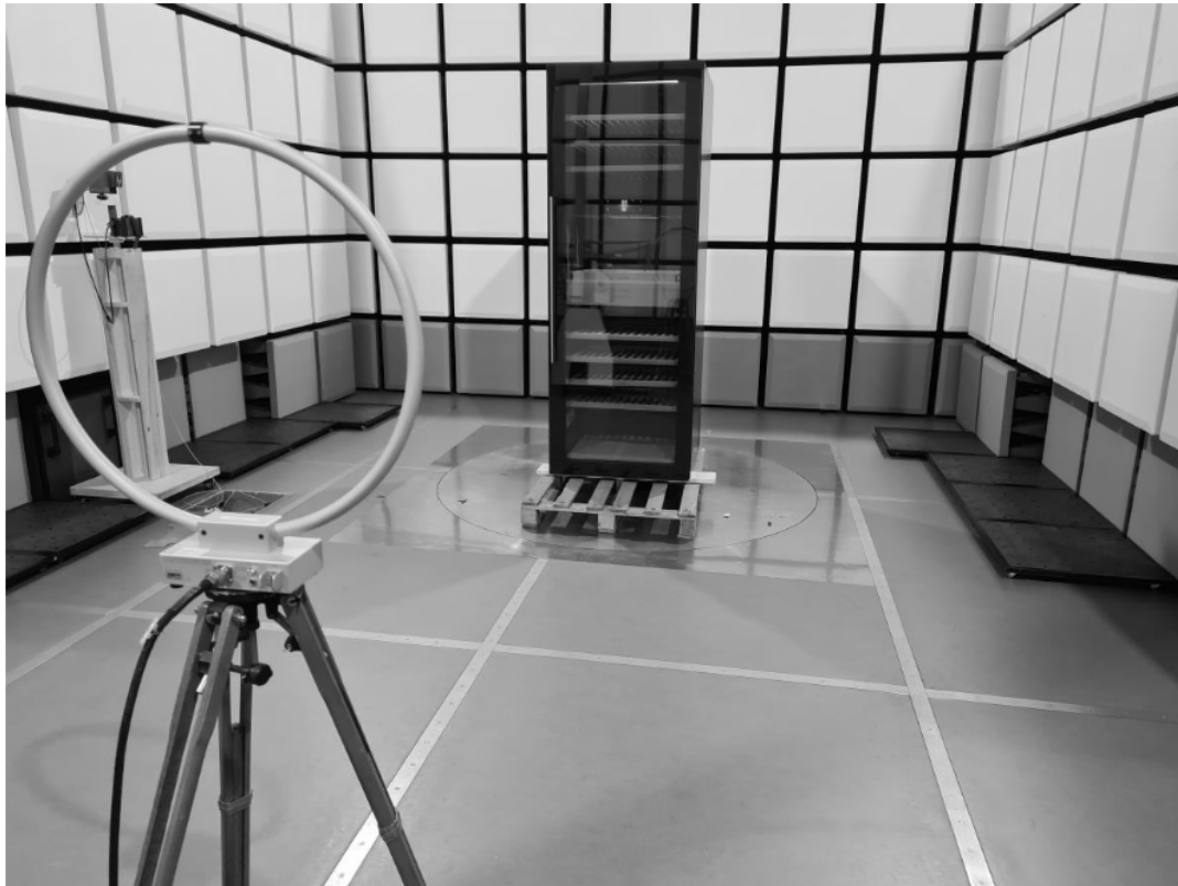
Figure 1: Spurious emission 9 kHz - 30 MHz
