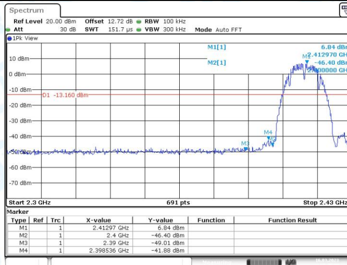
11B_Ant2_Low_2412
