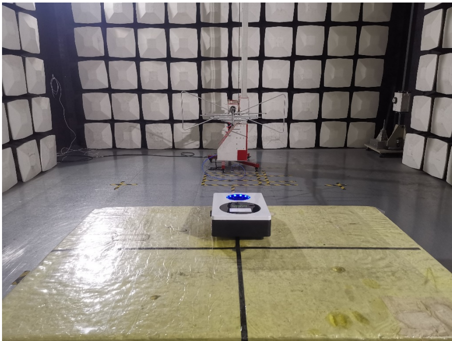
Set-up photo for Radiated Spurious Emission, 30MHz - 1GHz
