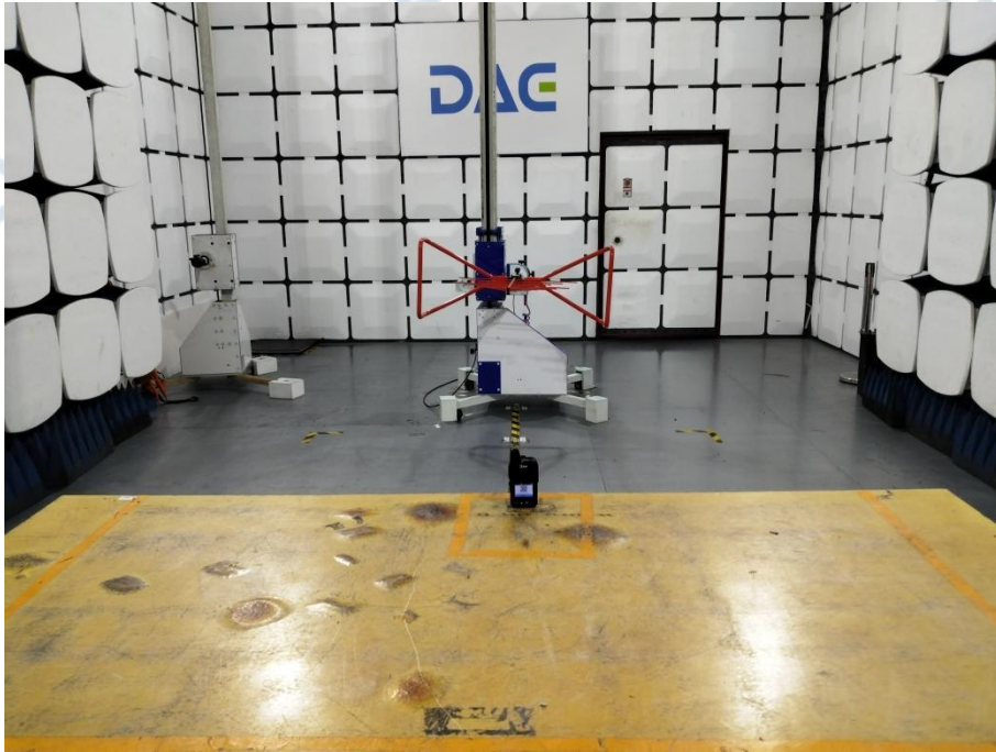
Spurious Unwanted Emission
