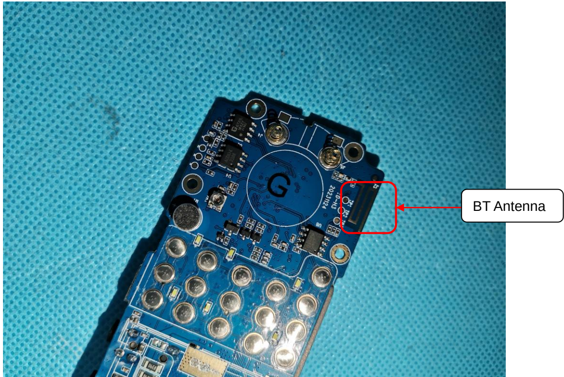
INTERNAL VIEW OF EUT (FIGURE 9)
