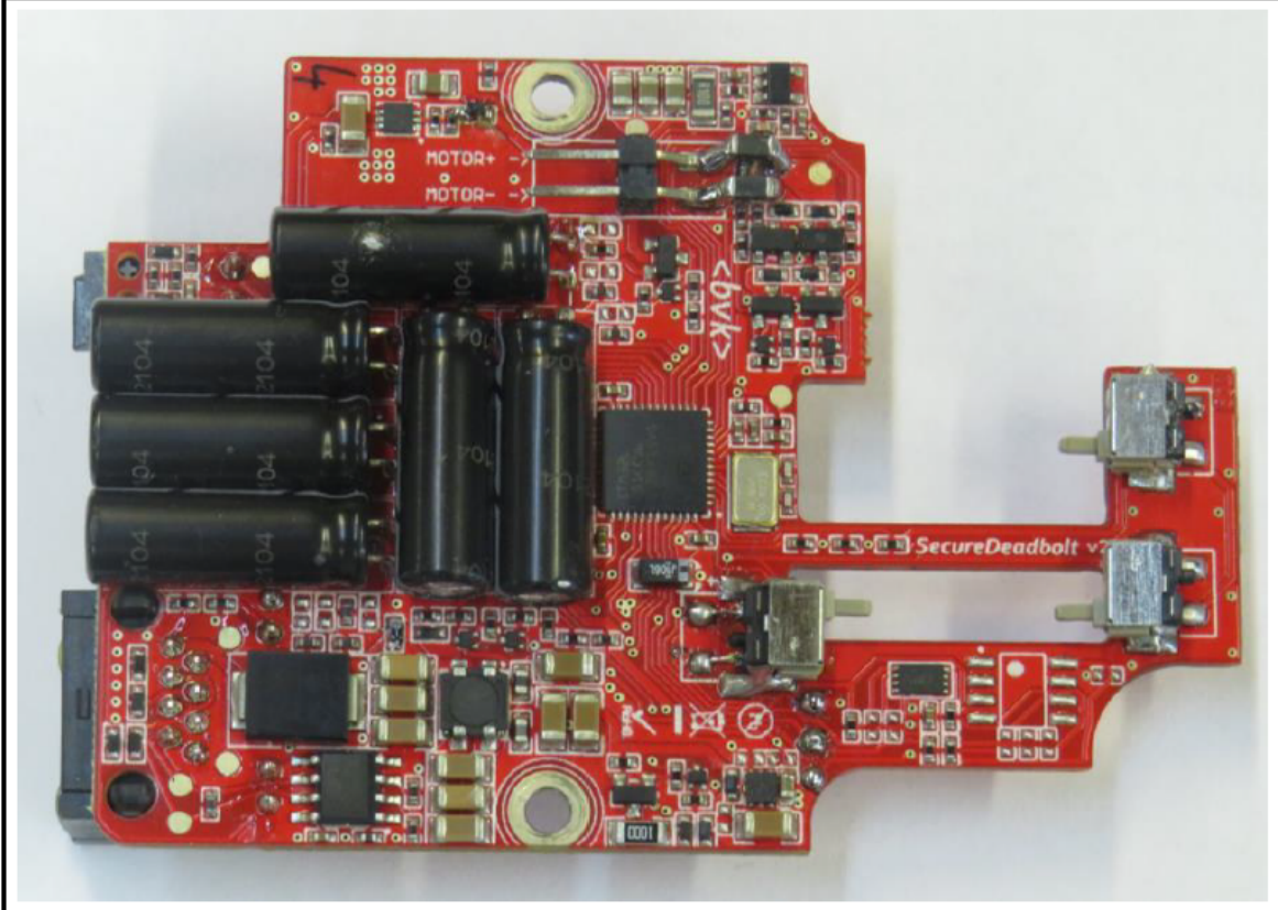
EUT PCB top view
