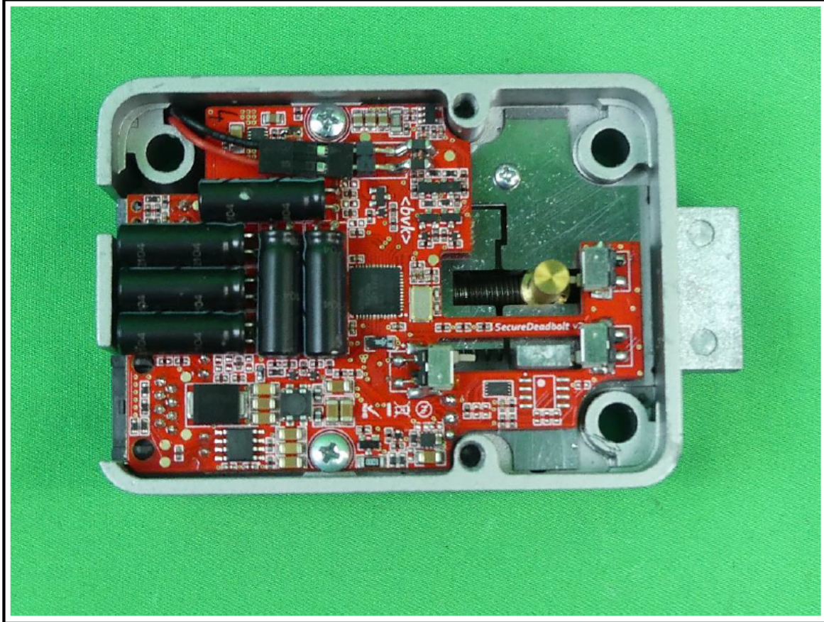
EUT with open housing view 1
