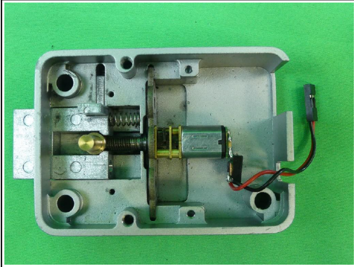
EUT with open housing view 2
