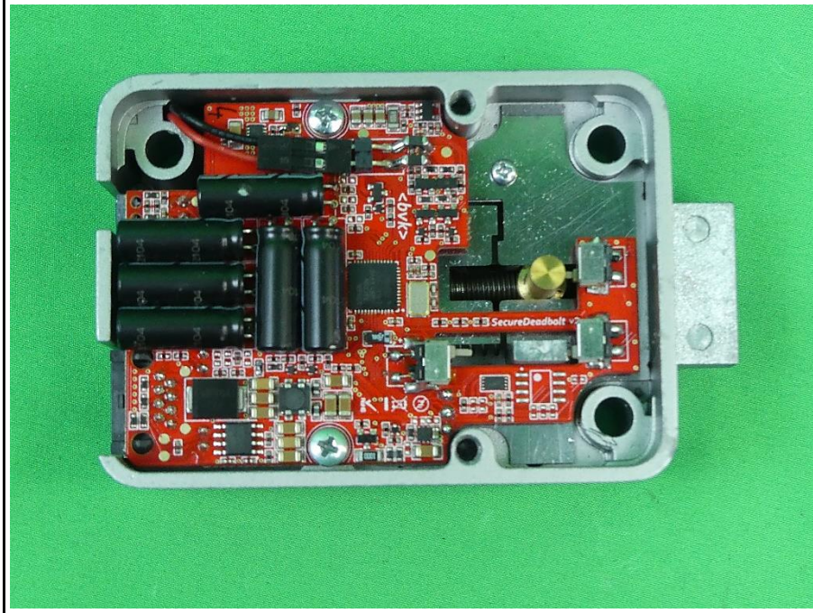
EUT with open housing view 1
