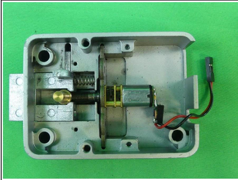
EUT with open housing view 2
