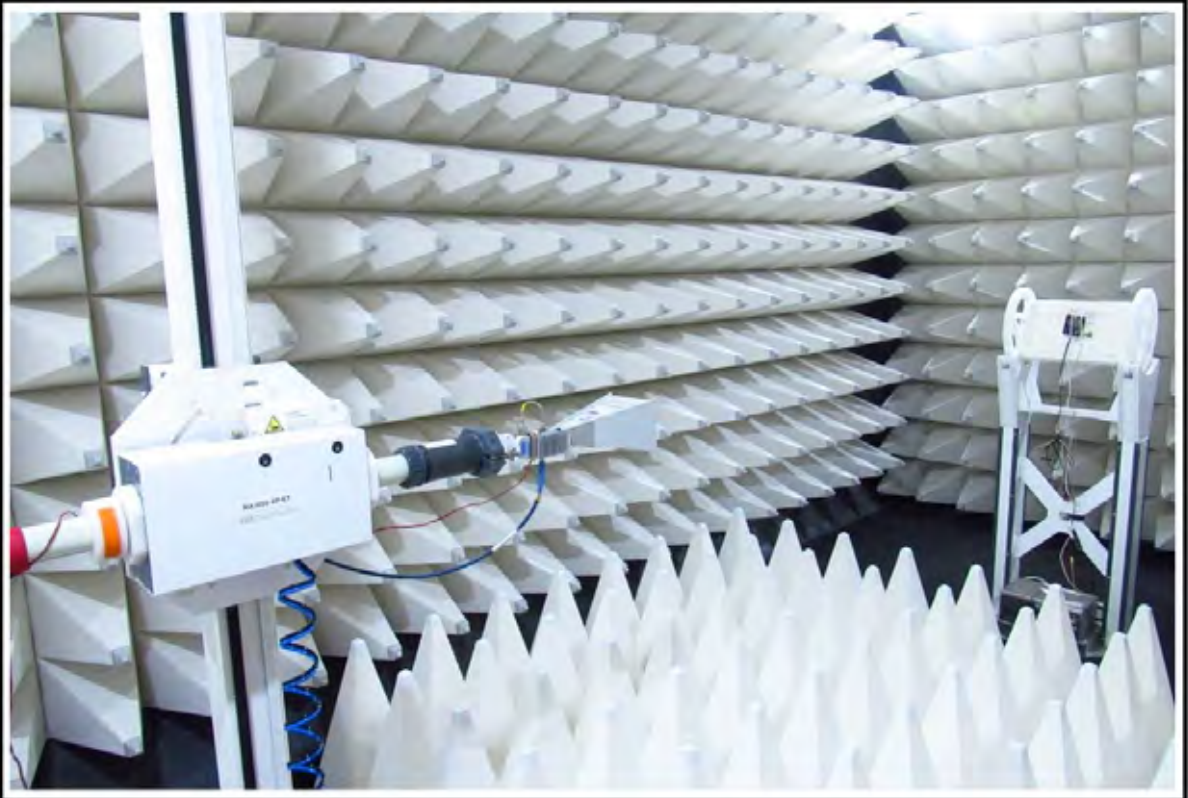
Setup above 1GHz
