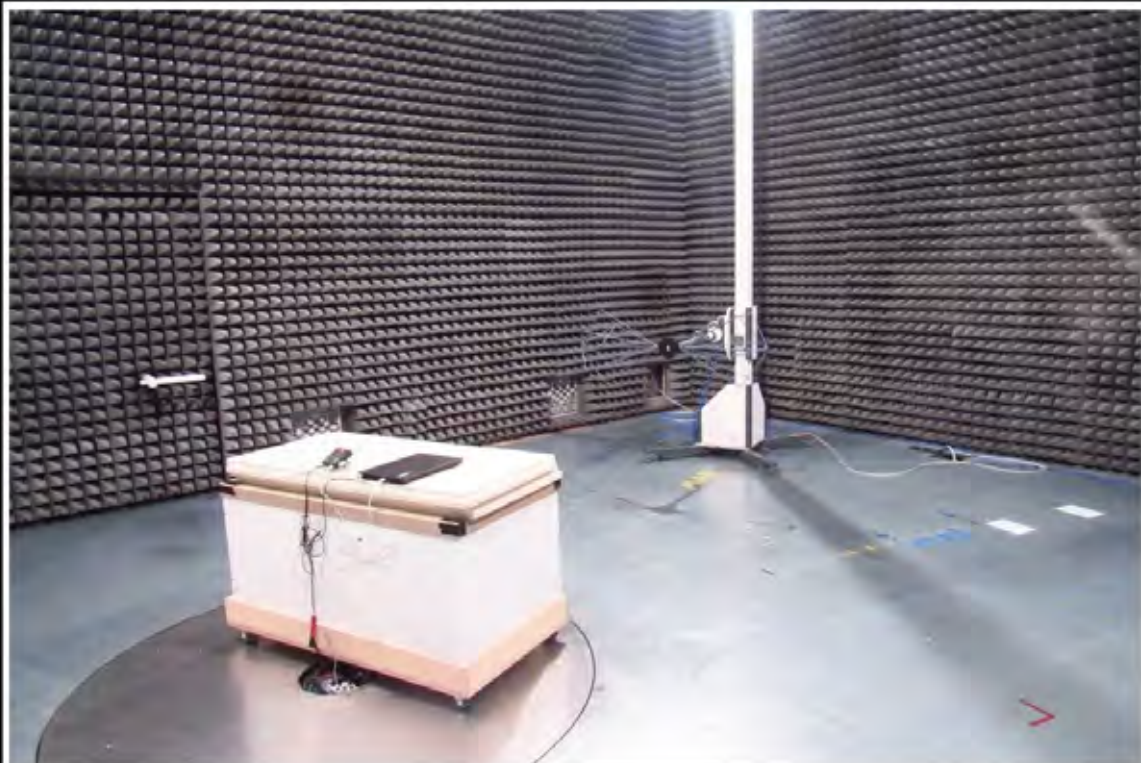
Setup below 1 GHz
