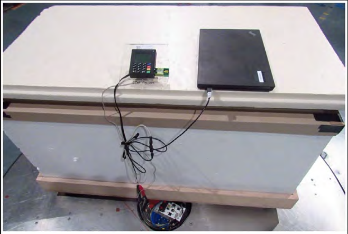
Setup EUT view below 1GHz
