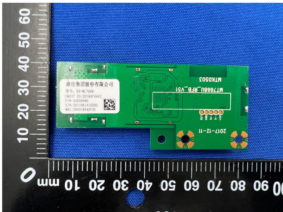
MAIN BOARD REAR VIEW MT7668
