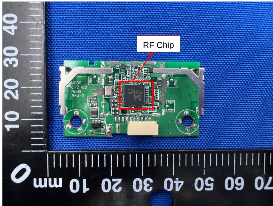
MAIN BOARD TOP VIEW (WITHOUT SHIELDING) RTL8812
