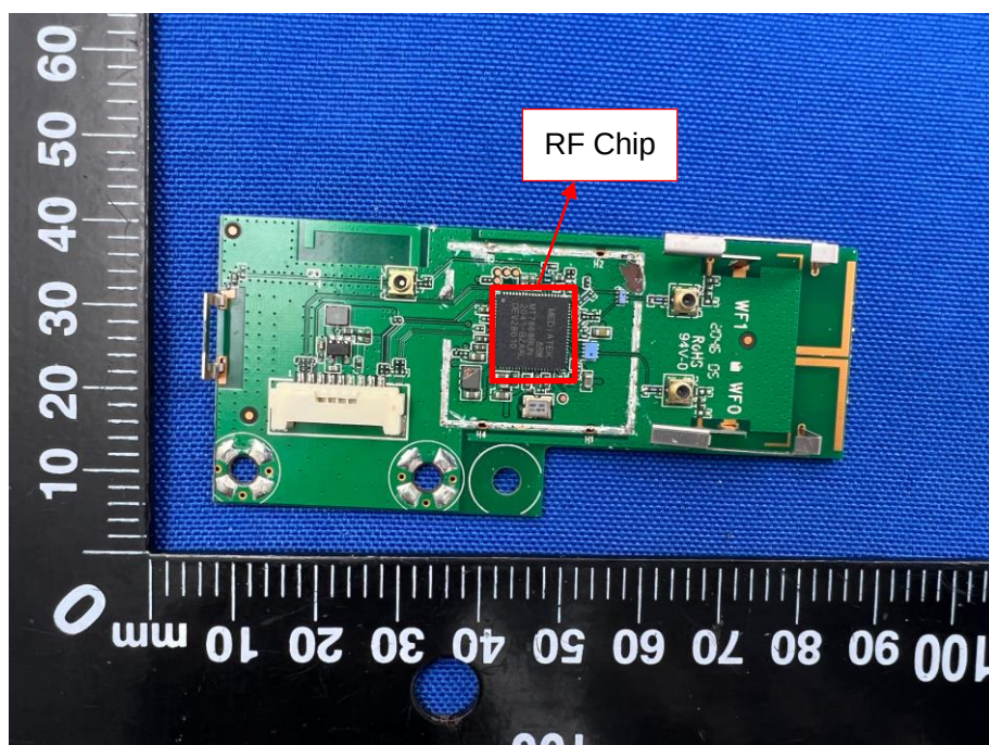
MAIN BOARD TOP VIEW (WITHOUT SHIELDING) MT7668
