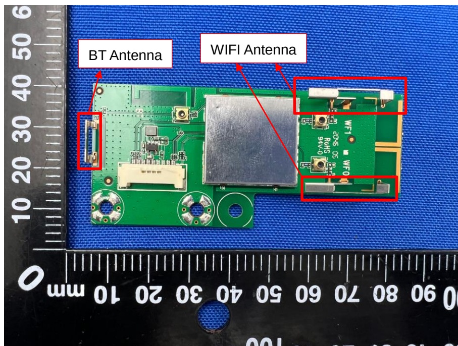
MAIN BOARD TOP VIEW (WITH SHIELDING) MT7668
