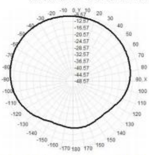
Total(H-XY), Max=-8.57dBi, CirD=12.97
