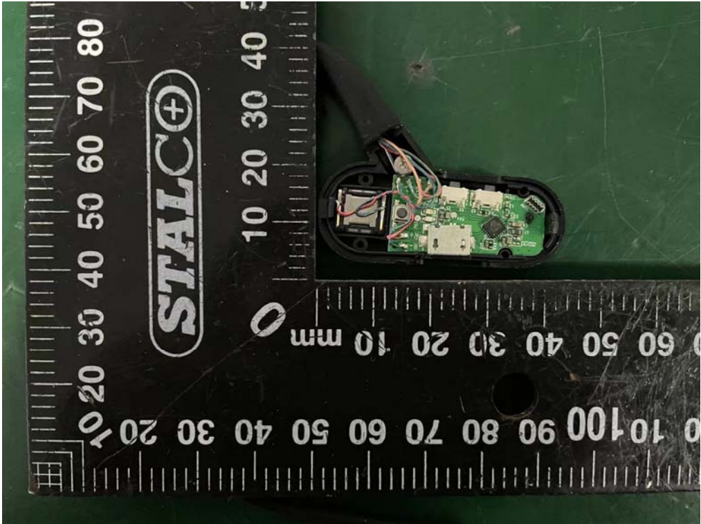
Internal Photos M/N: CGS-B6
