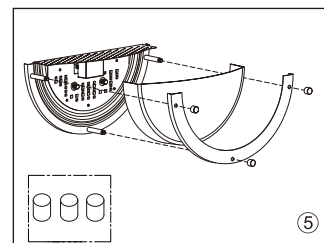
⑤ Tighten the thumb nuts on the metal ring to fix the LIGHT UNIT on wall firmly.
