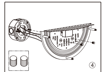
④ Approach LIGHT UNIT to the MOUNTING BRACKET CC, till LIGHT UNIT center hole aim on the screw of mounting bracket, fix LIGHT UNIT with round screw cap.
