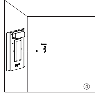
④ Approach LIGHT UNIT to the MOUNTING BRACKET CC, till LIGHT UNIT's center hole go through screw stem , adjust stem's length and tighten it with hex nut one, fix LIGHT UNIT with another hex nut two.
