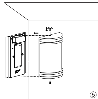
⑤ Put on fixture's shade and metal ring to fixture pan, fix them together with thumb nuts.
