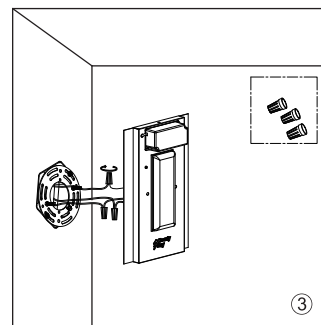
③ Pull out live wire, neutral wire and ground wire from junction box, connect live wire to LIGHT UNIT's black wire, connect neutral wire to LIGHT UNIT's white wire, connect ground wire to LIGHT UNIT's bare cooper wire with BB, or fix both ground wires on mounting bracket's green screw firmly.
