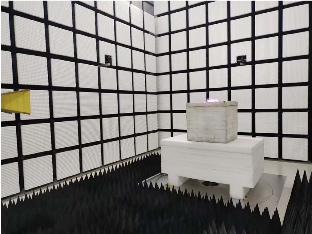
Radiated Emission Above 1GHz View LJD004BLWH
