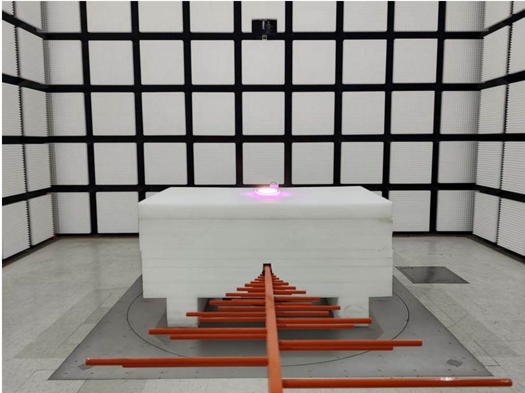
Radiated Emission Below 1GHz View LJD004BLWH
