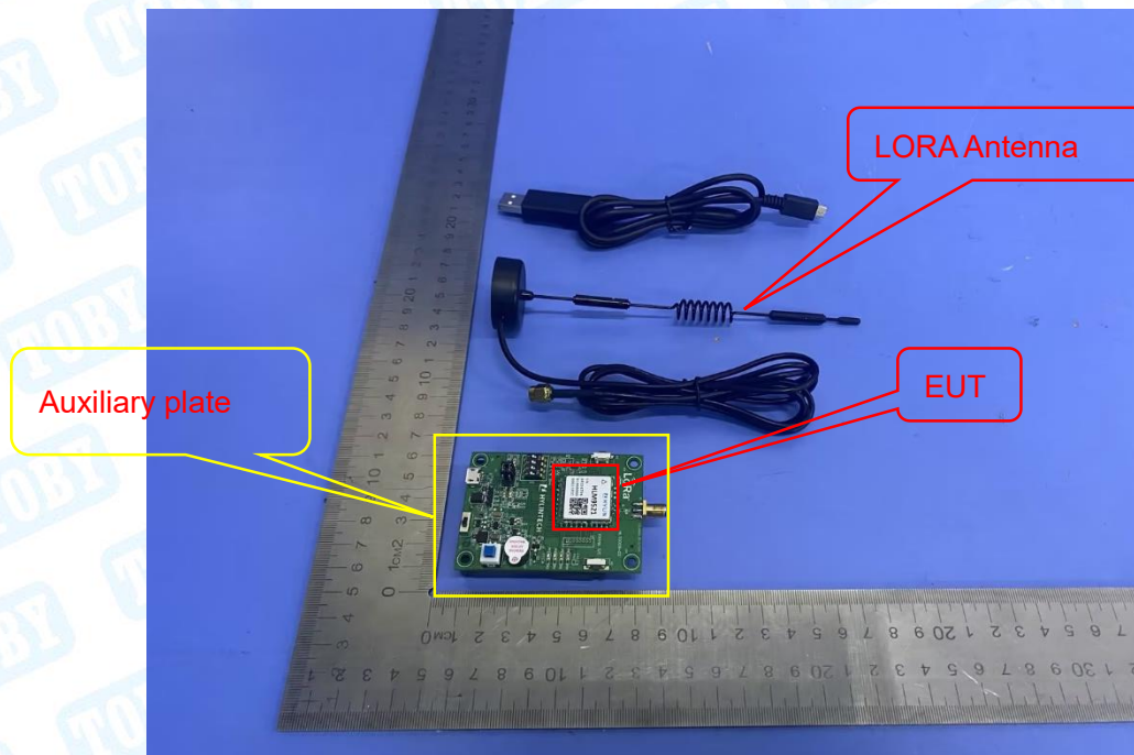
Photo 2 Appearance of EUT
