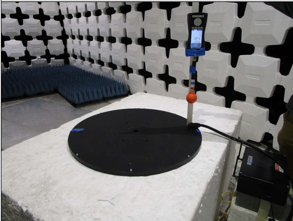
Test Setup for Nerve Stimulation Evaluation (TPM-SA-200-000)
