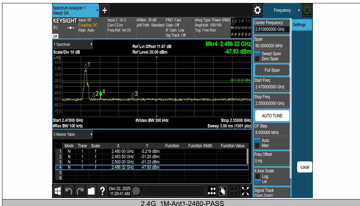
2.4G_1M-Ant1-2480-PASS
