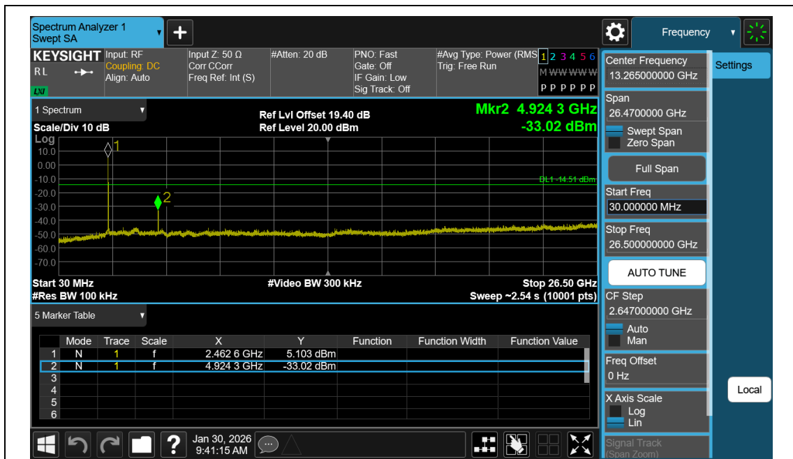
11B-Ant2-2462-30~26500-PASS
