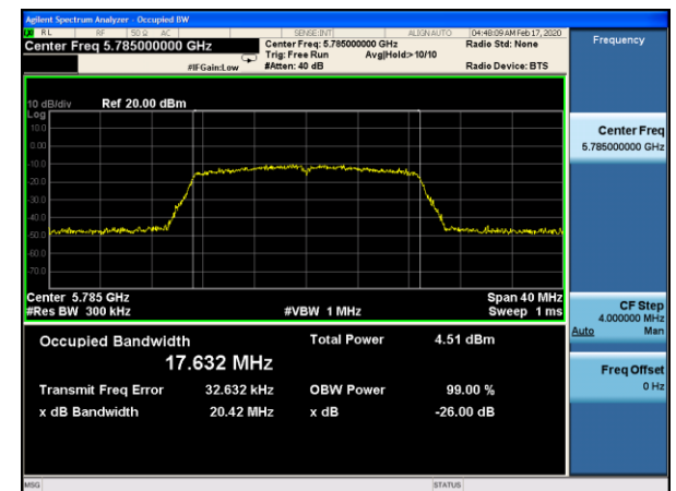
11ac (HT20) CH157
