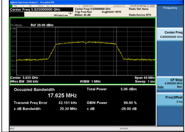
11a CH165
