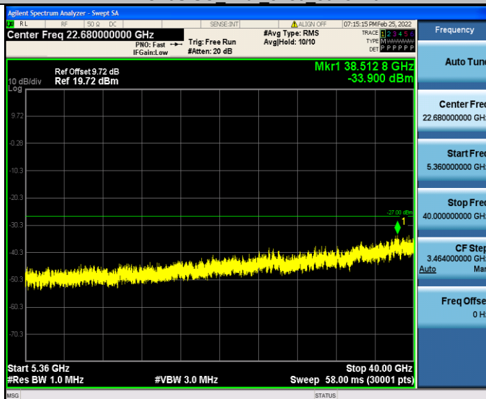
11AC40SISO Ant1 5230 5360~40000
