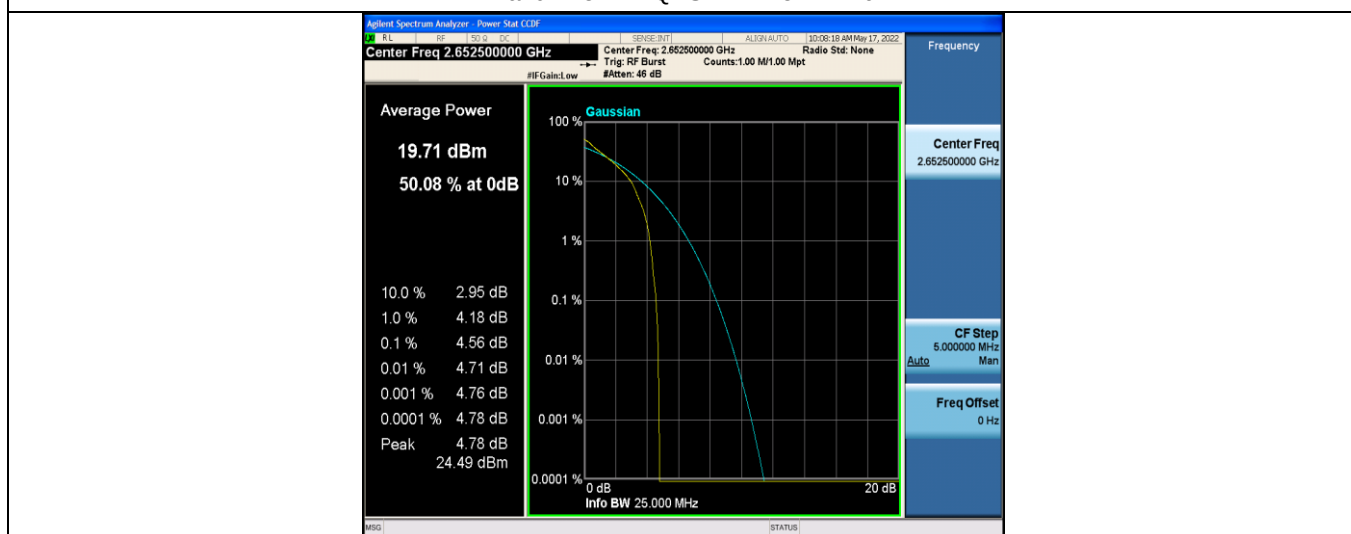
Band41-5MHz-QPSK-41215-25RB#0
