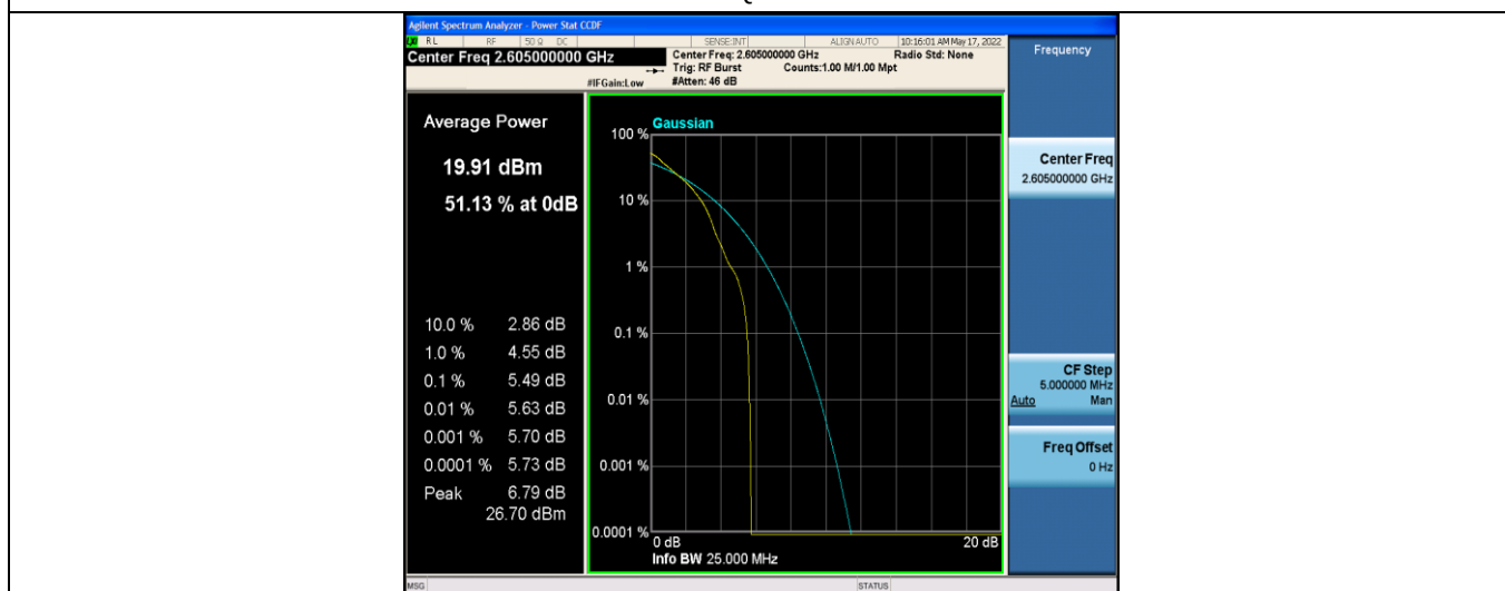
Band41-15MHz-QPSK-40740-75RB#0
