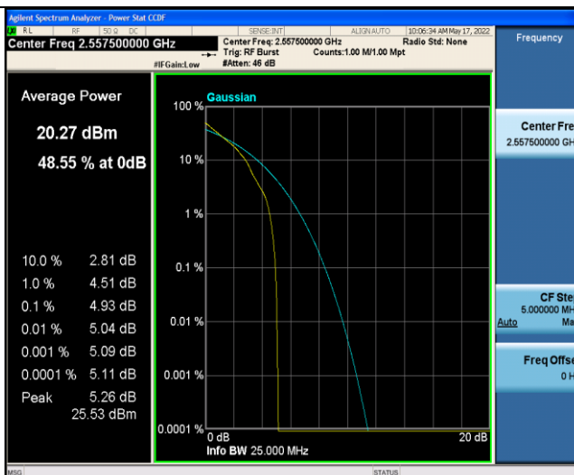
Band41-5MHz-QPSK-40265-25RB#0
