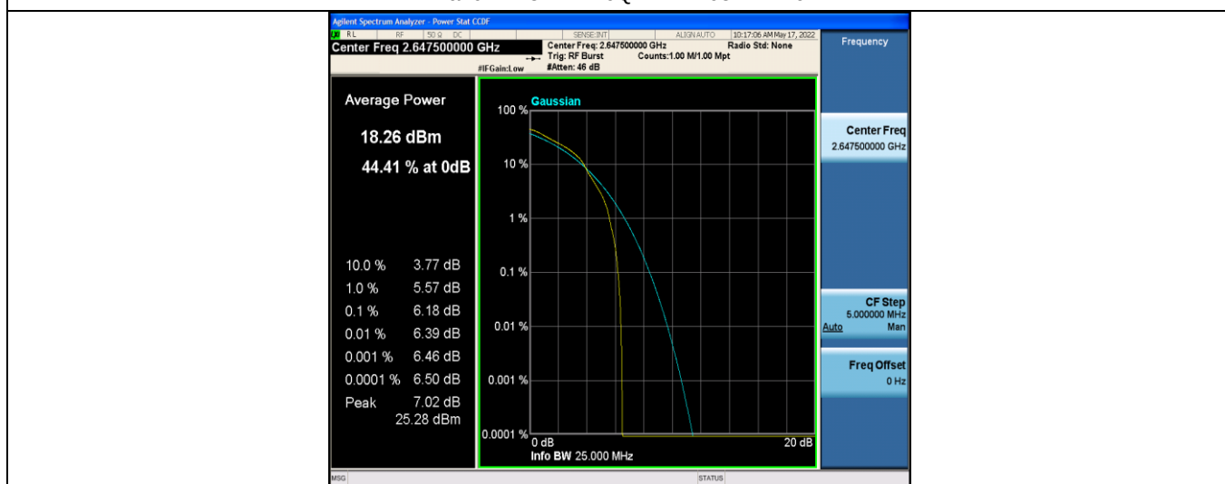
Band41-15MHz-16QAM-41165-75RB#0
