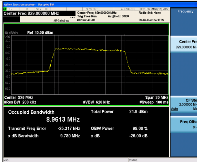
Band5-10MHz-QPSK-20525-50RB#0
