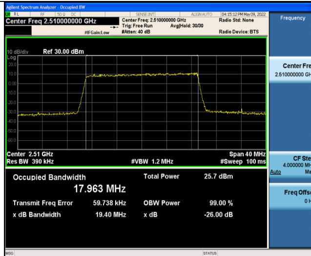
Band7-20MHz-16QAM-21100-100RB#0
