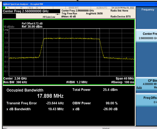
Band38-5MHz-QPSK-37775-25RB#0
