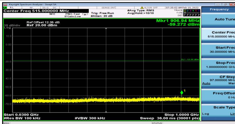
BLE_1M_Ant1_2402_30~1000
