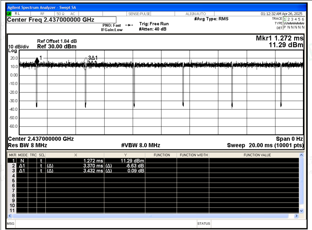
Duty Cycle NVNT ax20 2437MHz Ant2
