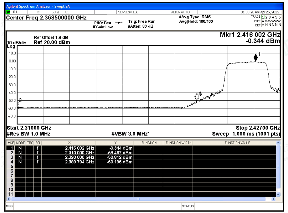
Restrict Band NVNT ax20 2412MHz Ant2 Average
