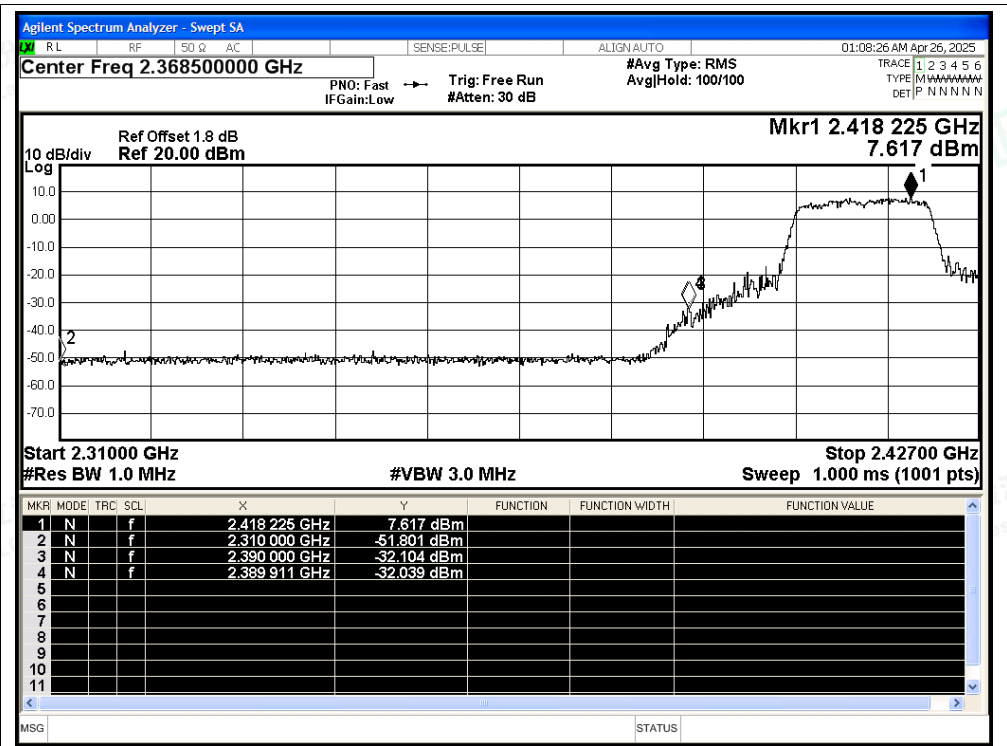
Restrict Band NVNT ax20 2412MHz Ant2 Average
