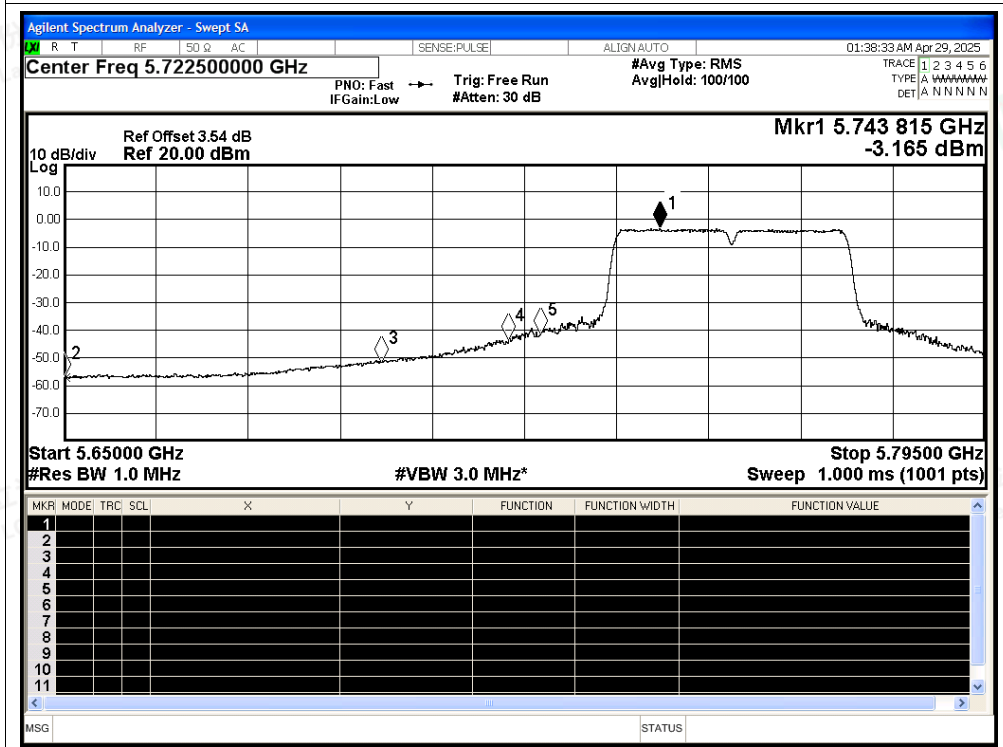
Restrict Band NVNT ax40 5755MHz Ant2 Average
