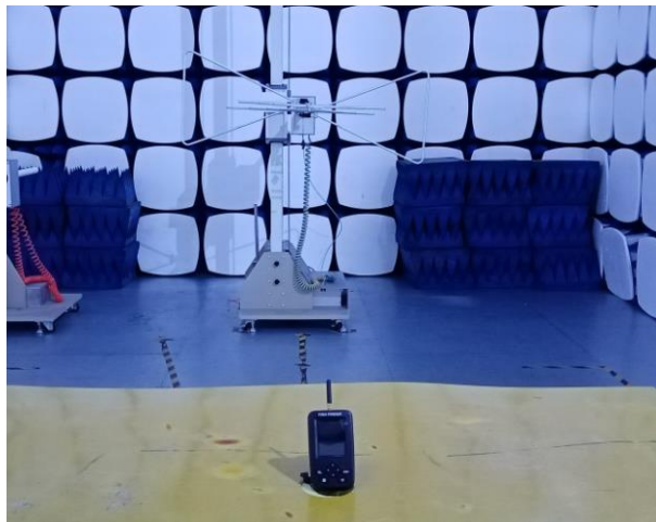
Radiated emission 30MHz~1GHz
